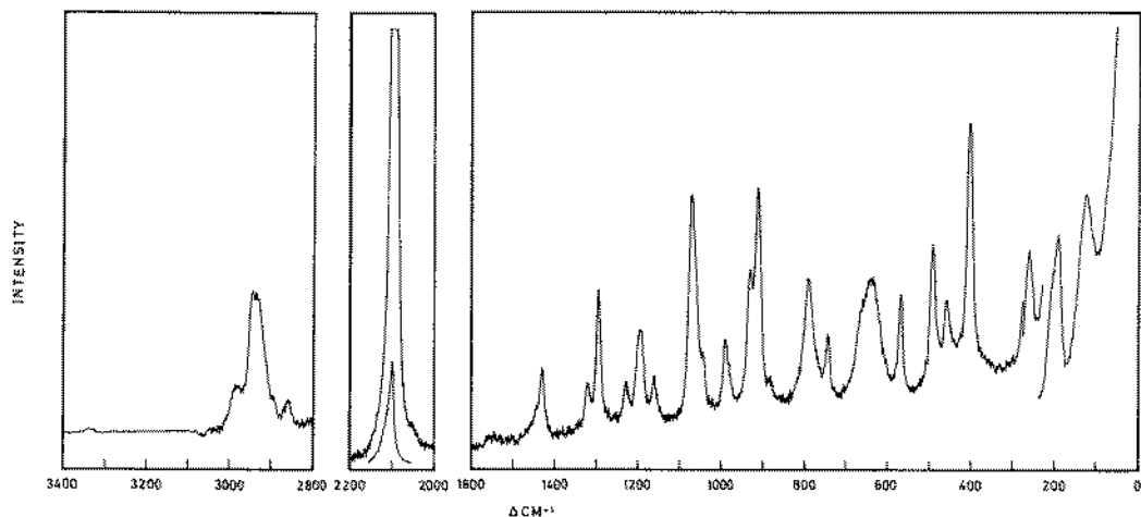
Fig. 3. Raman spectrum of cis -1,2-diethynylcyclobutane as a liquid.
