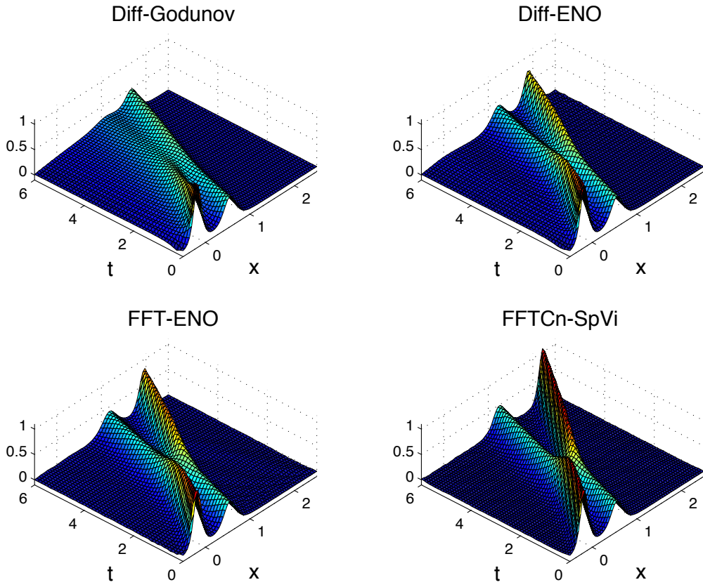
FIGURE 4. A two-soliton interaction
