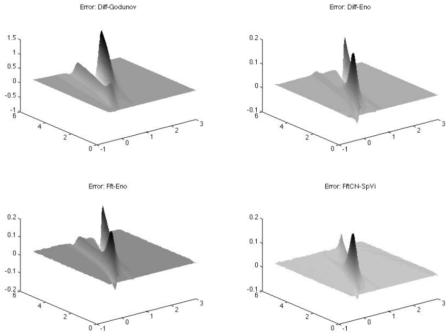
FIGURE 4. A two-soliton interaction
