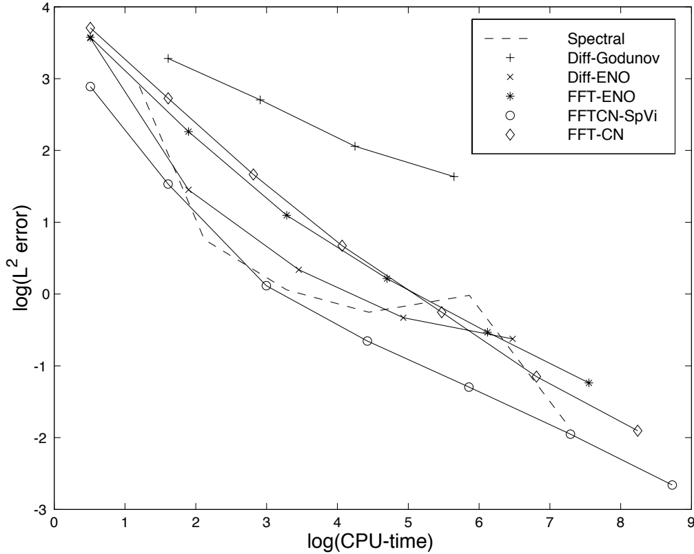
FIGURE 2. L^2 error vs. CPU-time
