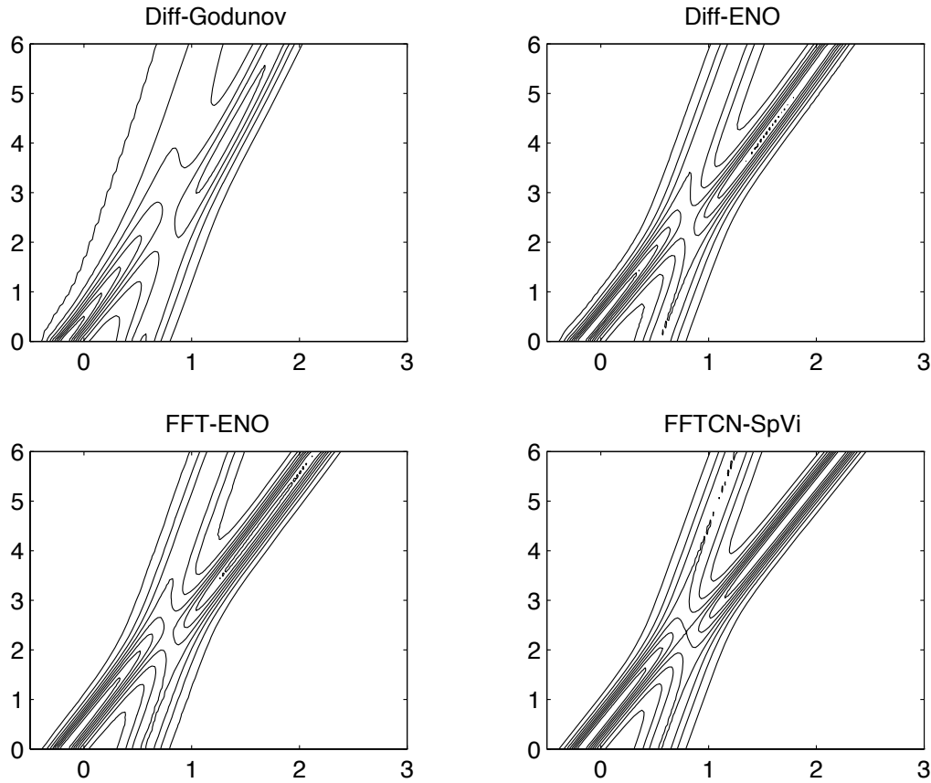
FIGURE 3. A two-soliton interaction
