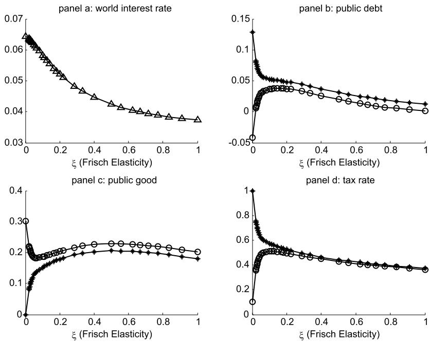
FIGURE 2.—Continuity of the SMPPE. Panel a plots the (annualized) equilibrium interest rate for economies with Frisch elasticity of labor supply \xi , ranging from 0 to 1. All other parameters are as given in Table I. Panels b, c, and d plot the corresponding steady-state allocations of debt, public goods, and taxes. The line with stars (circles) denotes the low- \theta (high- \theta ) economies. Stars and circles indicate the 24 values of \xi for which the SSMPPE is computed numerically. The values for \xi = 0 correspond to the equilibrium computed analytically in Proposition 1.
