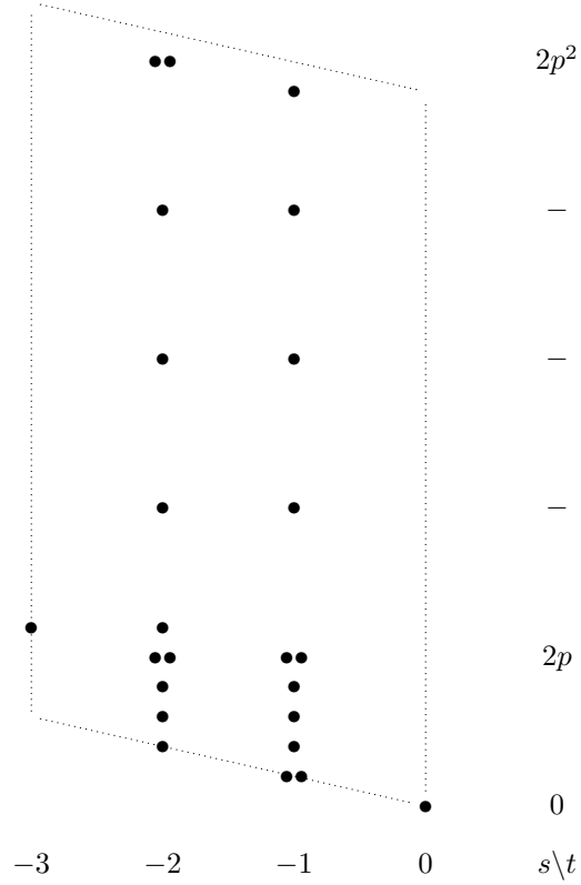
Figure 1. \mathbb{F}_p[v_2] -generators of E_{s,t}^2 = H_{\text{mot}}^{-s}(L_p; \mathbb{F}_{p^2}(t/2)) \implies V(1)_{s+t}K(L_p)
